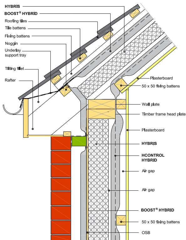
HY11 - Eaves details
