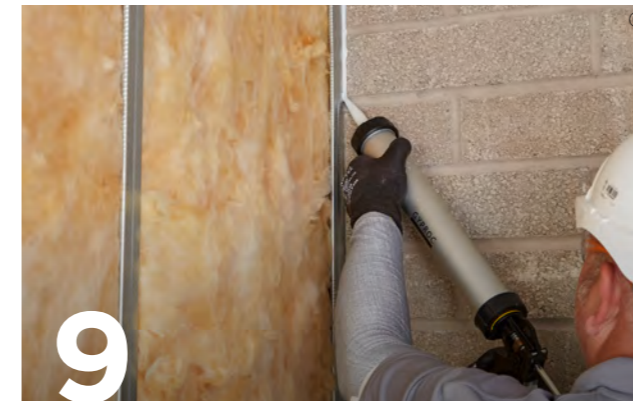
9 Use Gyproc Sealant to seal the perimeter of the partition except on the side where Gypframe RB1 Resilient Bars are to be installed. Where Gypframe RB1 Resilient Bars are to be installed, the Gyproc Sealant is applied to the perimeter of the first layer of board.
