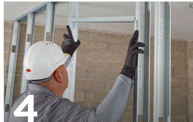
4 Construct door openings to suit the partitions' duty rating.
