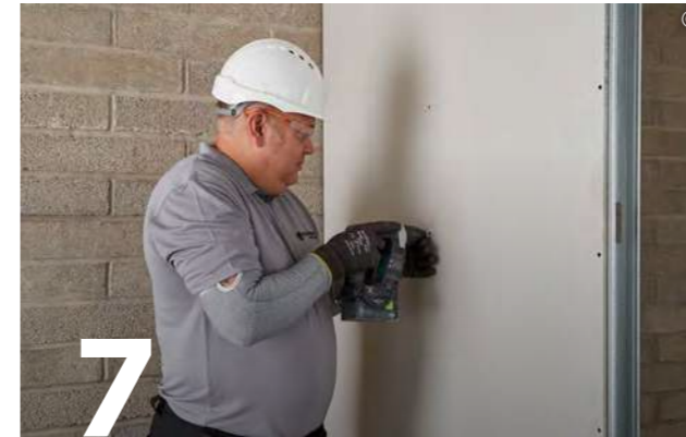
7 Use British Gypsum Drywall Screws to fix Gyproc DuraLine (and Gyproc SoundBloc inner layer if required) plasterboards to the Gypframe framework.
