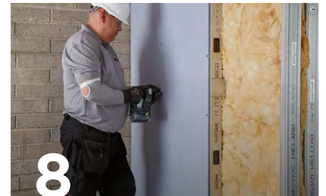
Use British Gypsum Drywall Screws to fix Gyproc plasterboards to the Gypframe framework.
