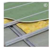
GypCeiling Shaft Lightweight, fire resistant structure to protect elements in confined spaces wherever access is limited to one side only. See page 10.3.
