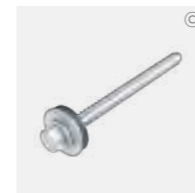
Stainless steel self-drilling insulation fastener screws (4.8 mm diameter) Use to attach Polterm Max Plus into the SFS framework. Minimum 10mm threaded penetration into the SFS framework.
