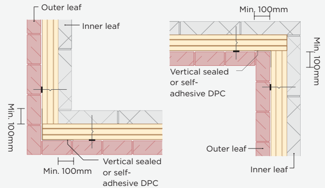
FIGURE 4 - EXTERNAL CORNER DETAIL
