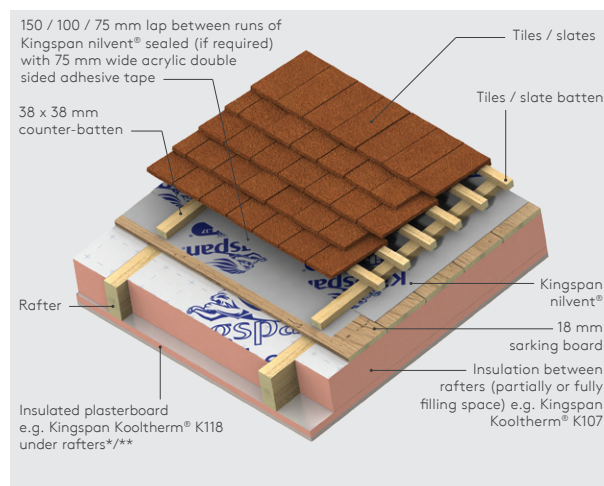
Figure 1c - Insulation between rafters - sarking board - battens & tiles
