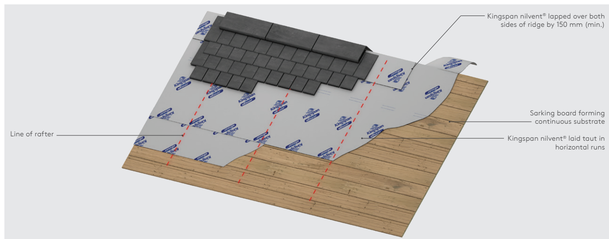
Figure 5f - Ridge - fully supported horizontal installation with natural slates
