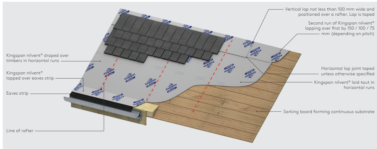
Figure 5d - Eaves - fully supported horizontal installation with natural slates
