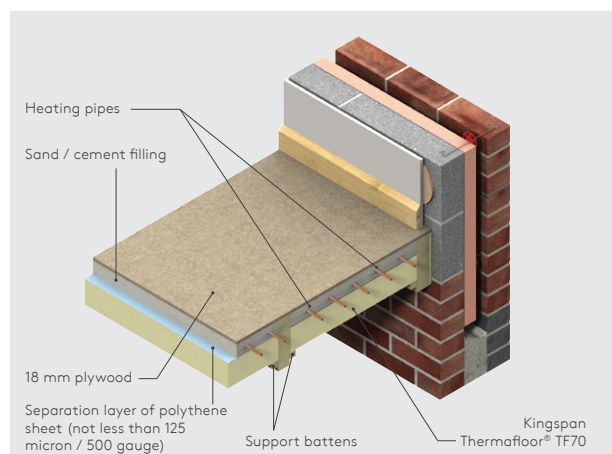
Figure 14 - Intermittent heating applications - suspended timber floor
