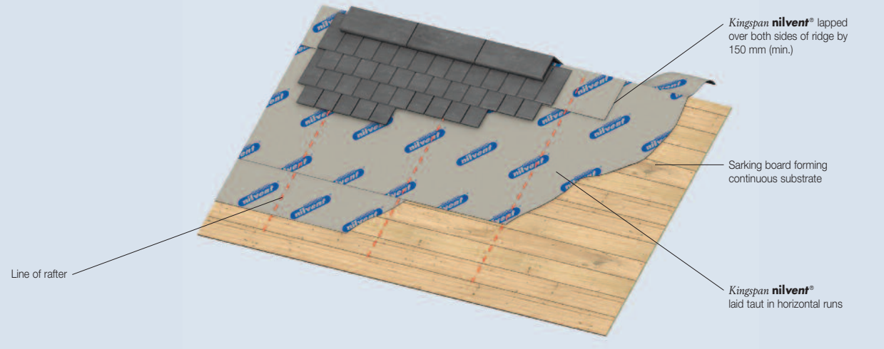
Figure 5d Ridge – Fully Supported Horizontal Installation with Natural Slates
