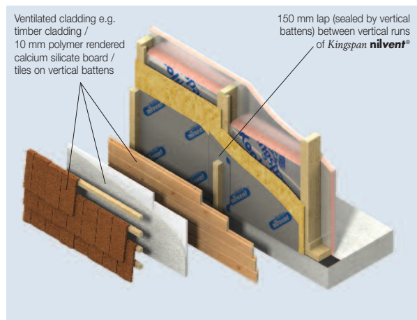
Figure 5b – Ventilating Cladding
