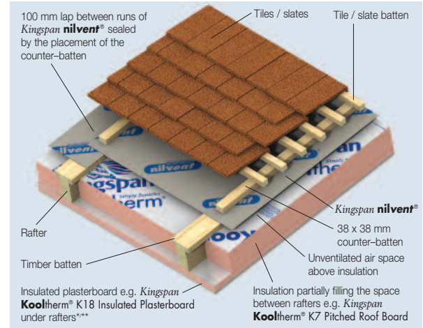
Figure 2a – Partially Filled Insulation Between Rafters – No Sarking Board – Battens & Tiles
