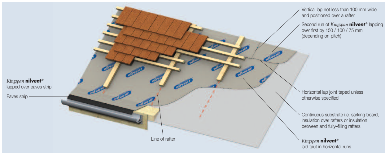
Figure 5a Eaves – Fully Supported Horizontal Installation
