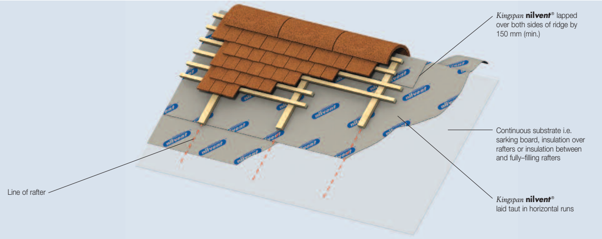
Figure 5c Ridge – Fully Supported Horizontal Installation
