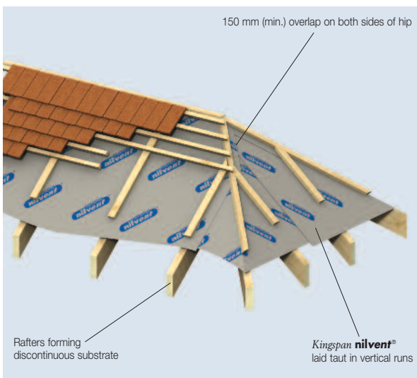
10c Hips – Vertical Installation
