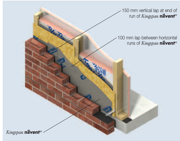
Figure 4a – External Masonry
