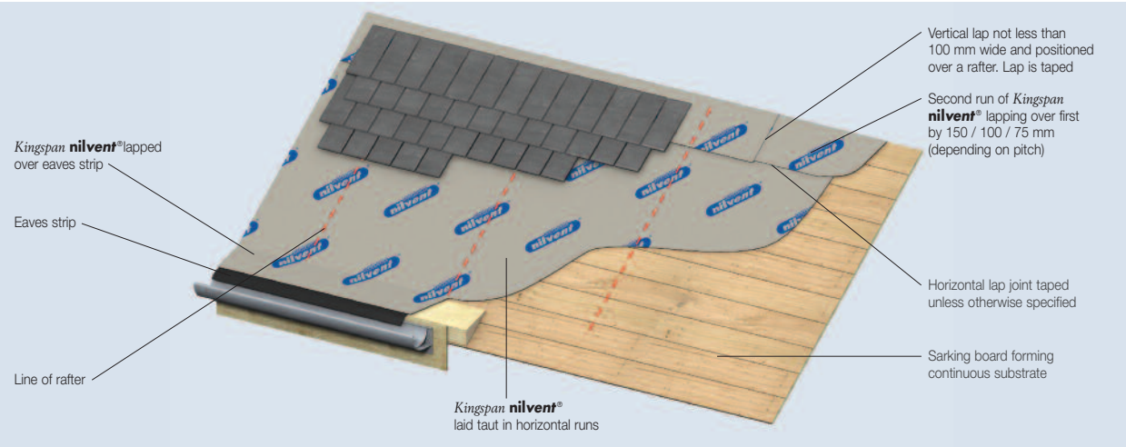
Figure 5b Eaves – Fully Supported Horizontal Installation with Natural Slates
