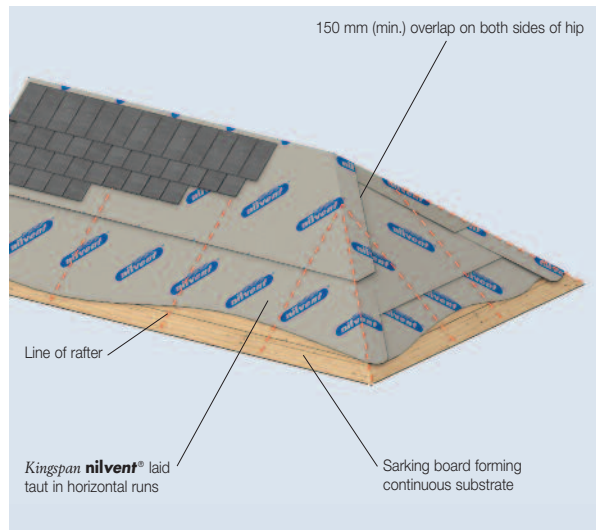
Figure 10b Hips – Fully Supported Horizontal Installation with Natural Slates
