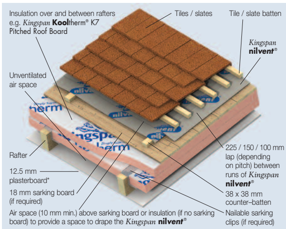
Figure 3b – Insulation Over Rafters – Sarking Board / No Sarking Board – Battens & Tiles
