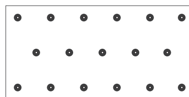
17 No. per board (2.4 x 1.2 m board - 5.90 fixings / m 2 )
