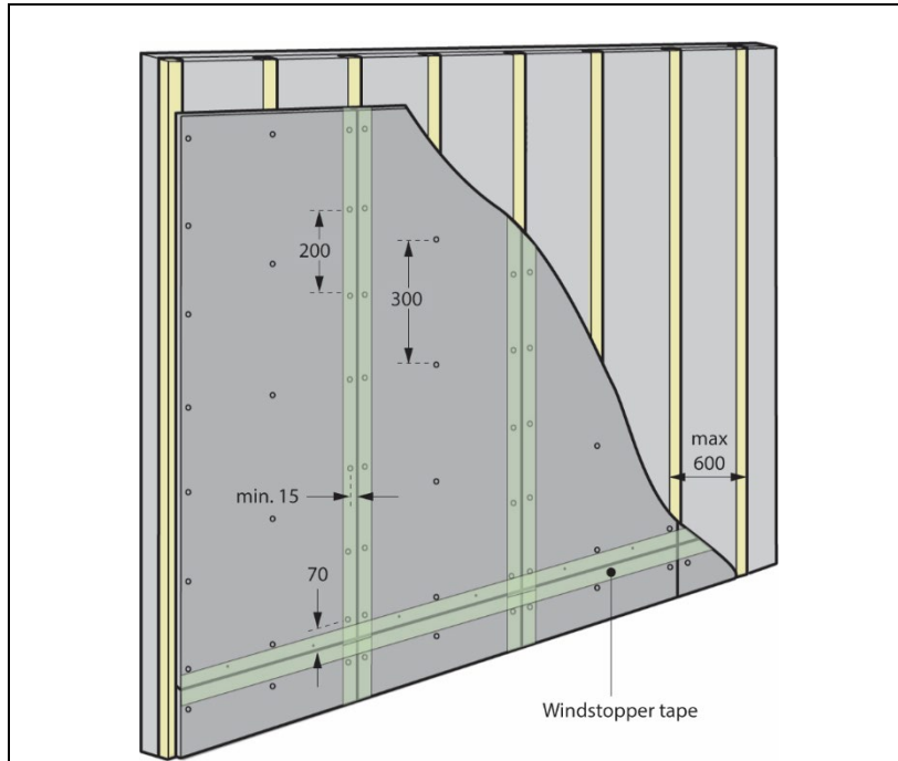
Figure 2 Board installation, vertical orientation (all dimensions in mm)
